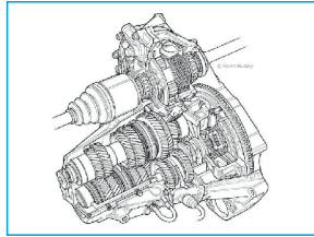
Transmission
